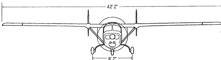
Figure 1-1 Three View
